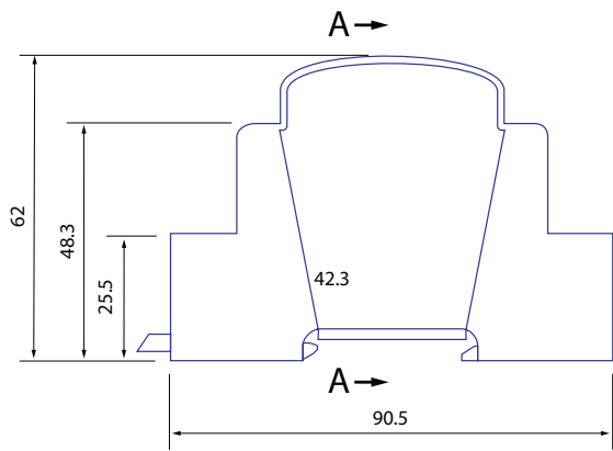
Figure 2: Side View
