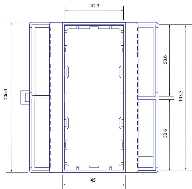
Figure 1: Top View
